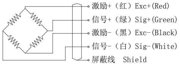
接线图Wiring Schematic Diagram
